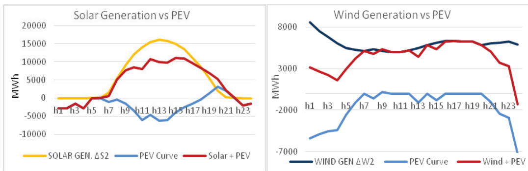
Fig. 5: PEV generation-consumption vs a) solar and b) wind generation
